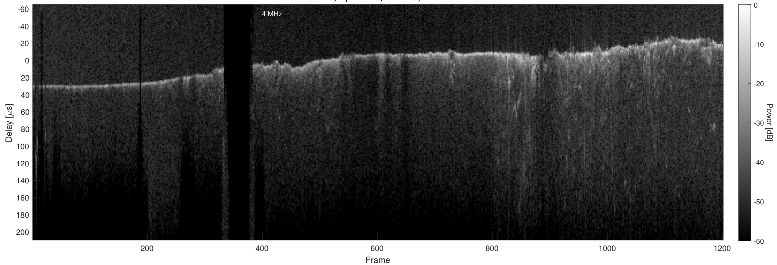
Orbit 2977, Optimized, Window, Channel 2
