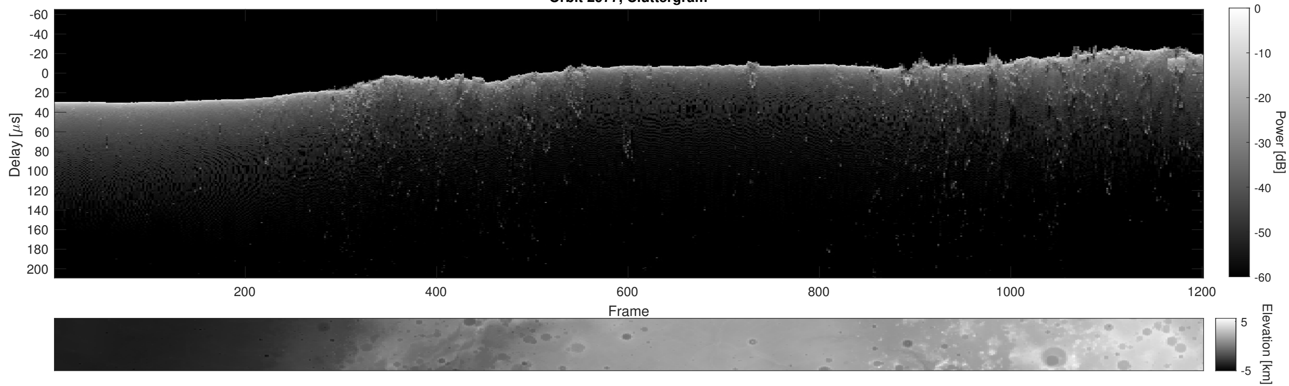
Orbit 2977, Cluttergram
