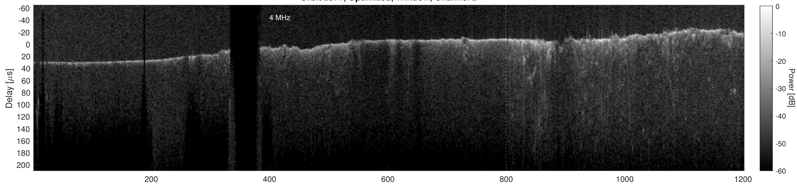
Orbit 2977, Cluttergram
