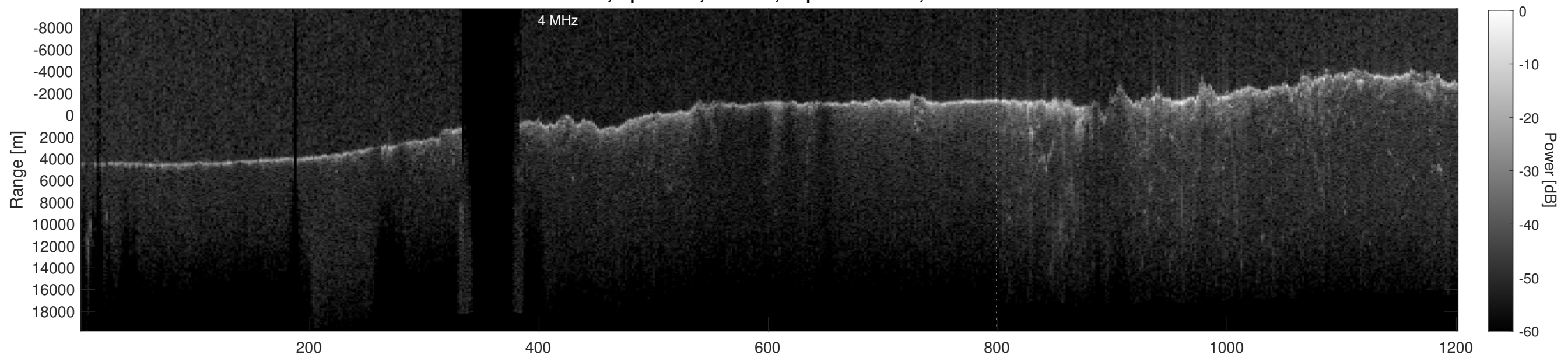
Orbit 2977, Depth-Corrected Cluttergram
