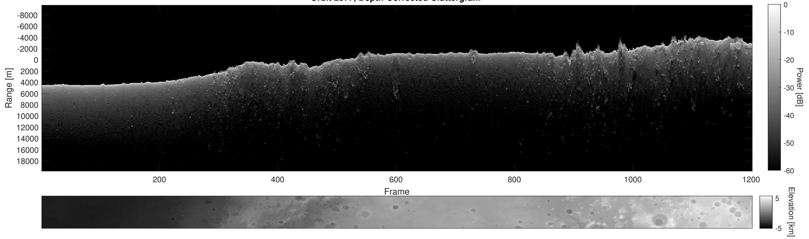
Orbit 2977, Depth-Corrected Cluttergram
