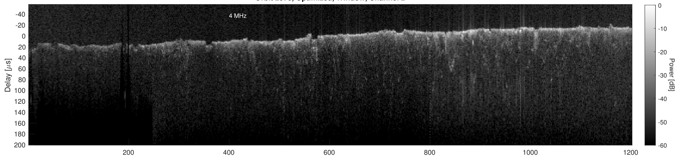
Orbit 2978, Cluttergram
