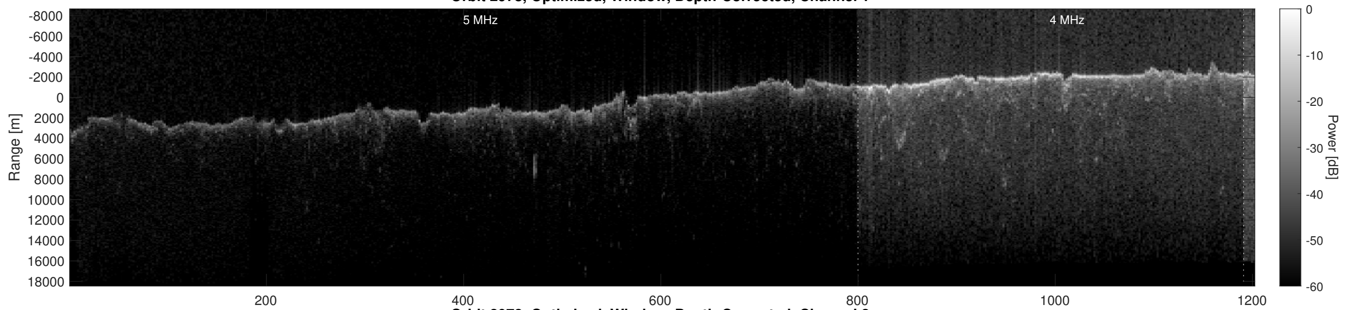
Orbit 2978, Optimized, Window, Depth-Corrected, Channel 2
