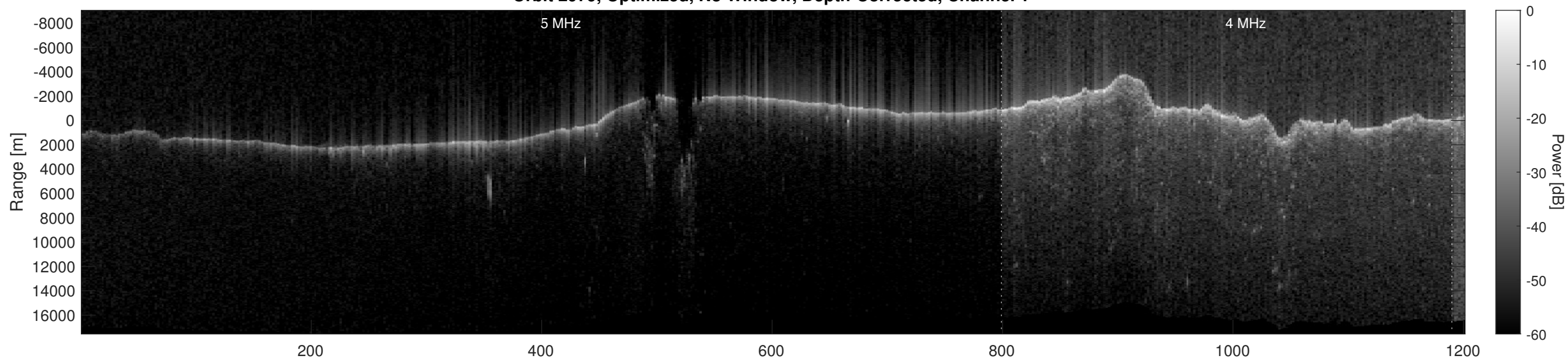
Orbit 2979, Optimized, No Window, Depth-Corrected, Channel 2
