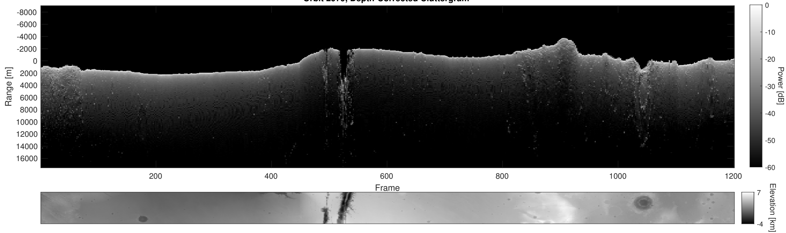
Orbit 2979, Depth-Corrected Cluttergram
