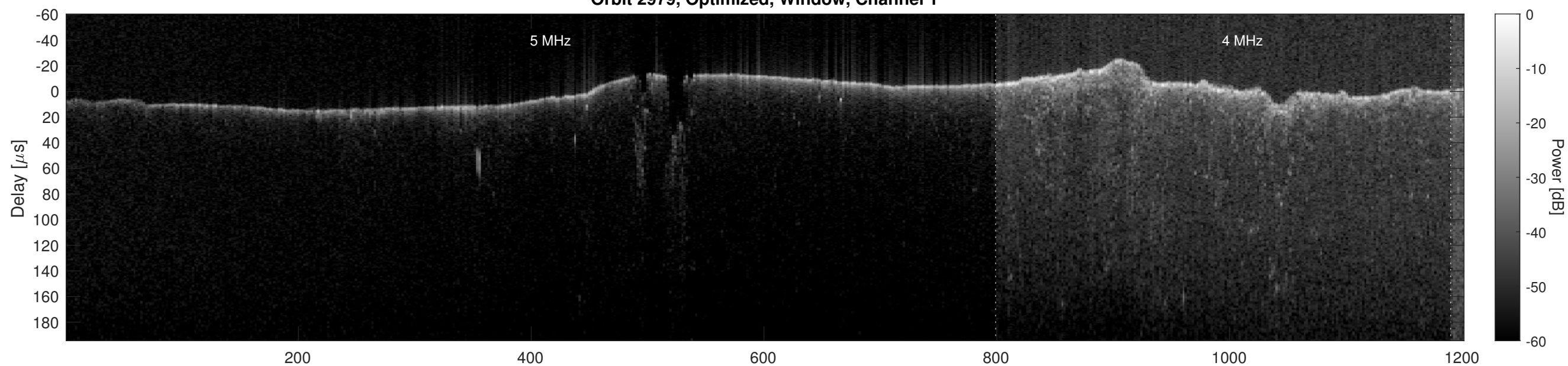
Orbit 2979, Optimized, Window, Channel 2
