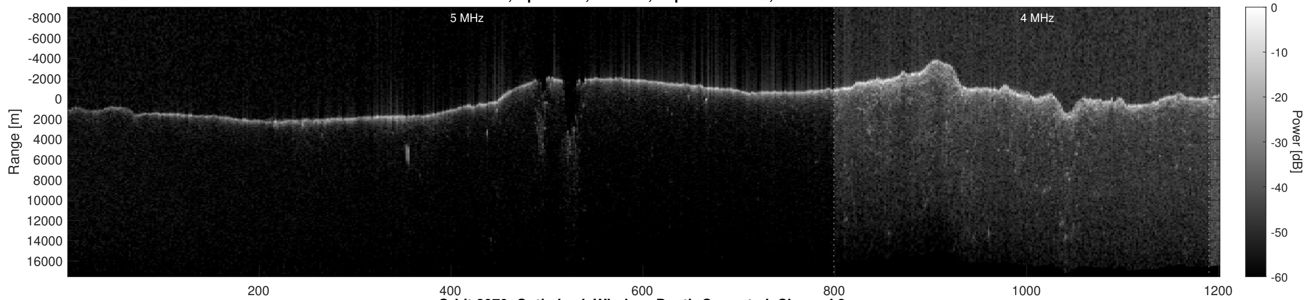
Orbit 2979, Optimized, Window, Depth-Corrected, Channel 2
