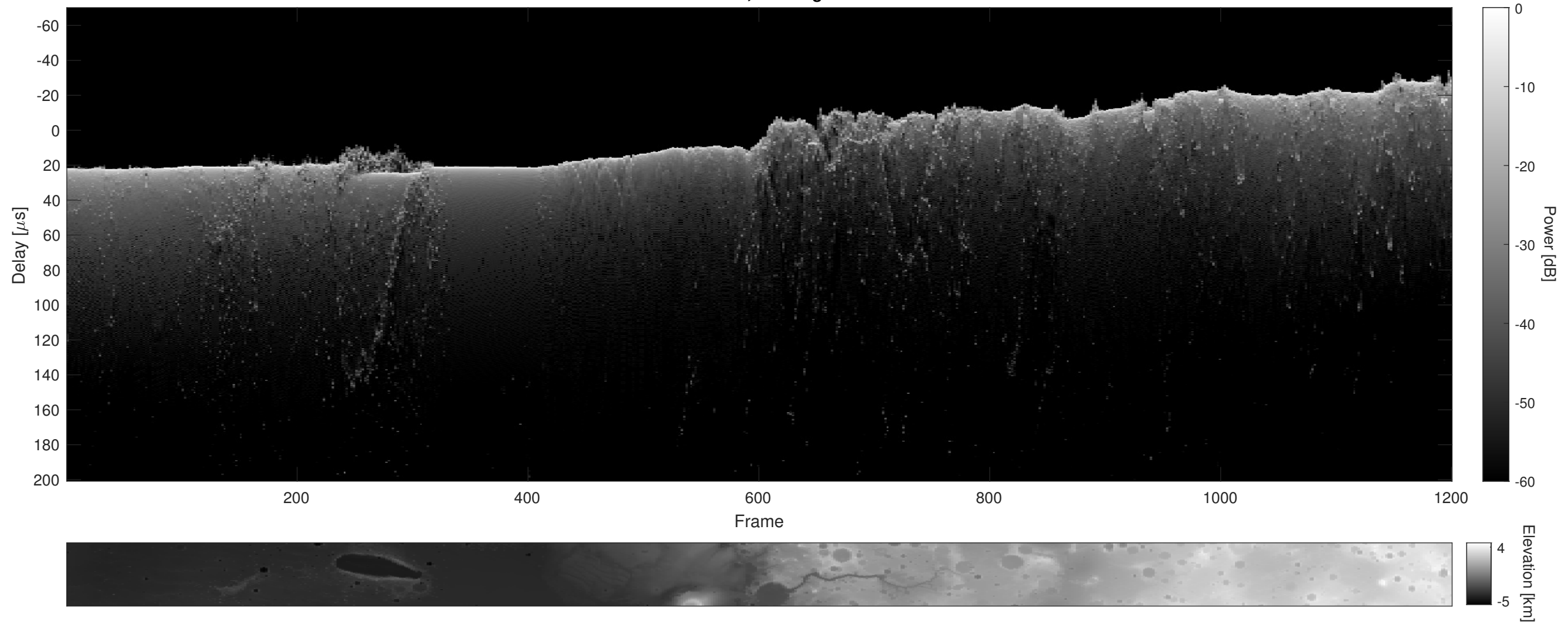
Orbit 2980, Cluttergram
