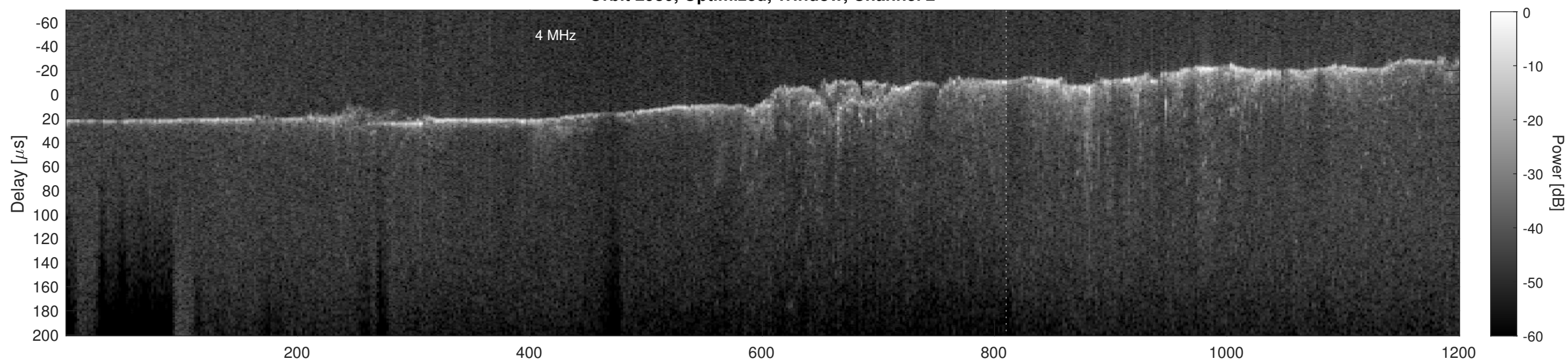
Orbit 2980, Cluttergram
