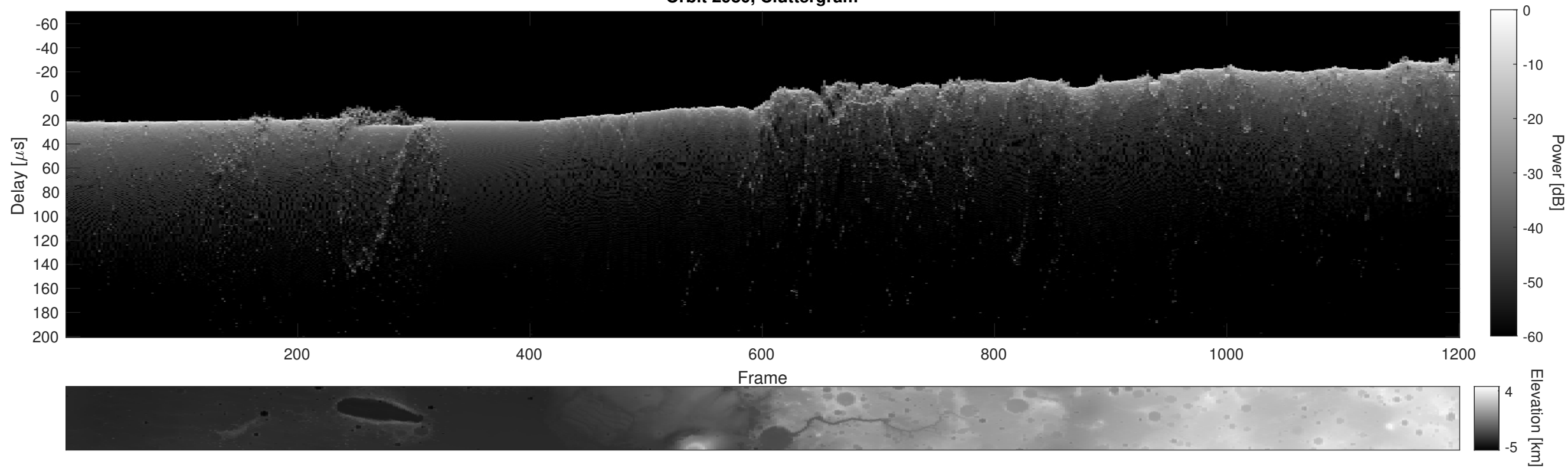
Orbit 2980, Cluttergram
