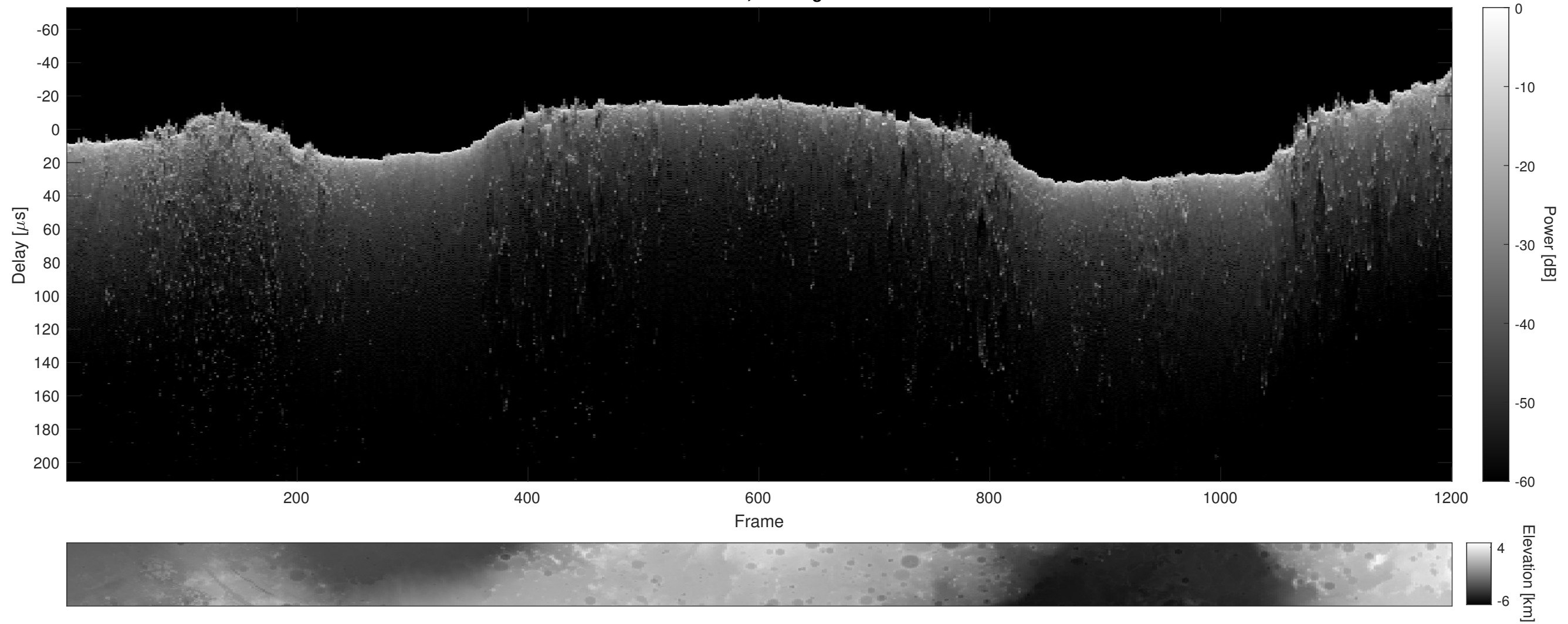
Orbit 2981, Cluttergram
