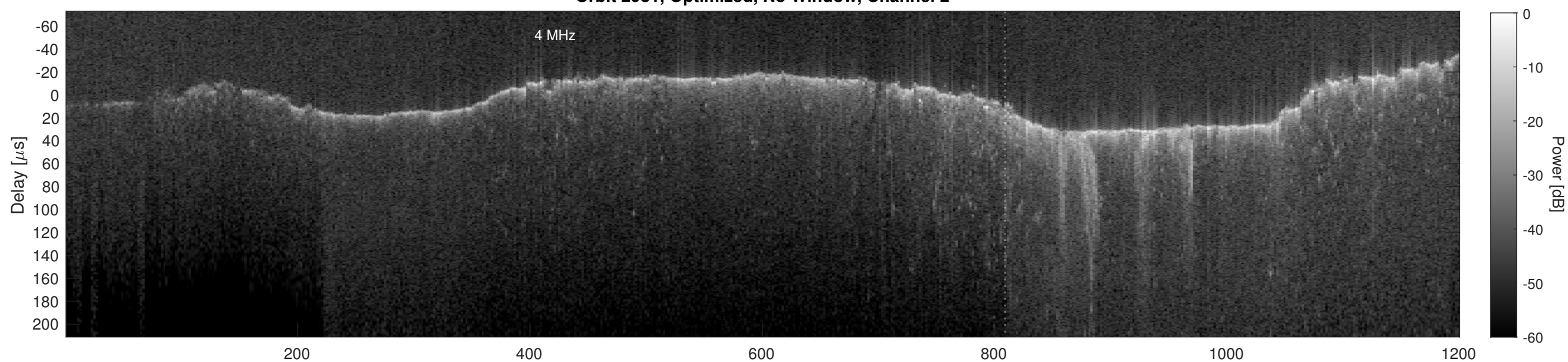
Orbit 2981, Cluttergram
