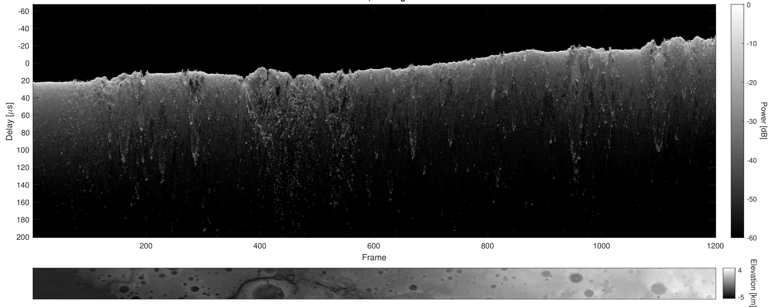
Orbit 2982, Cluttergram
