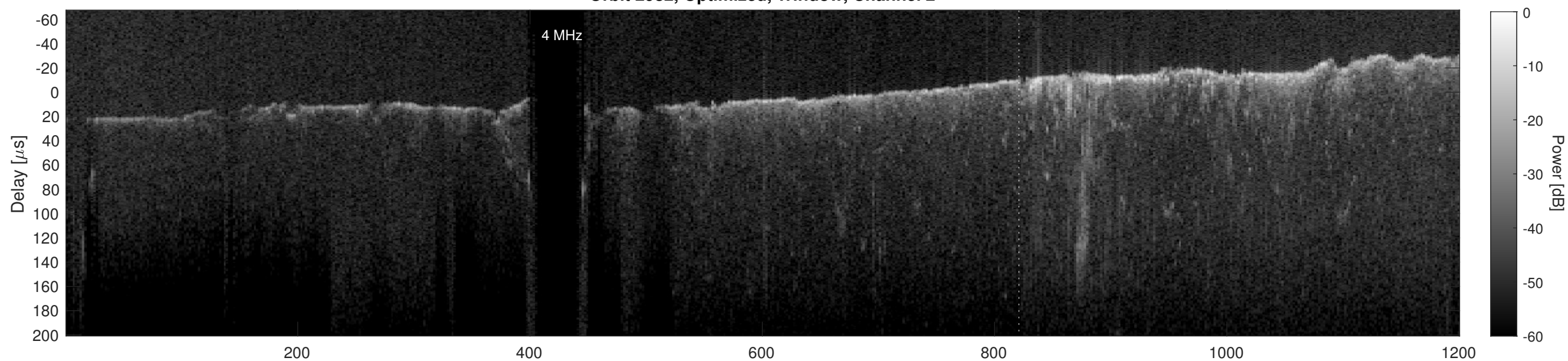
Orbit 2982, Cluttergram
