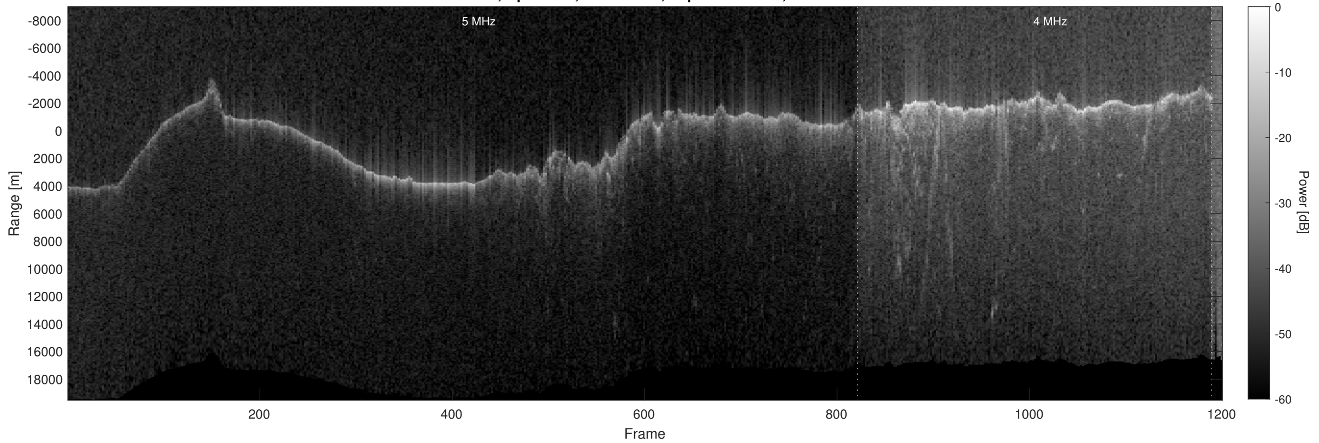
Orbit 2984, Optimized, No Window, Depth-Corrected, Channel 2
