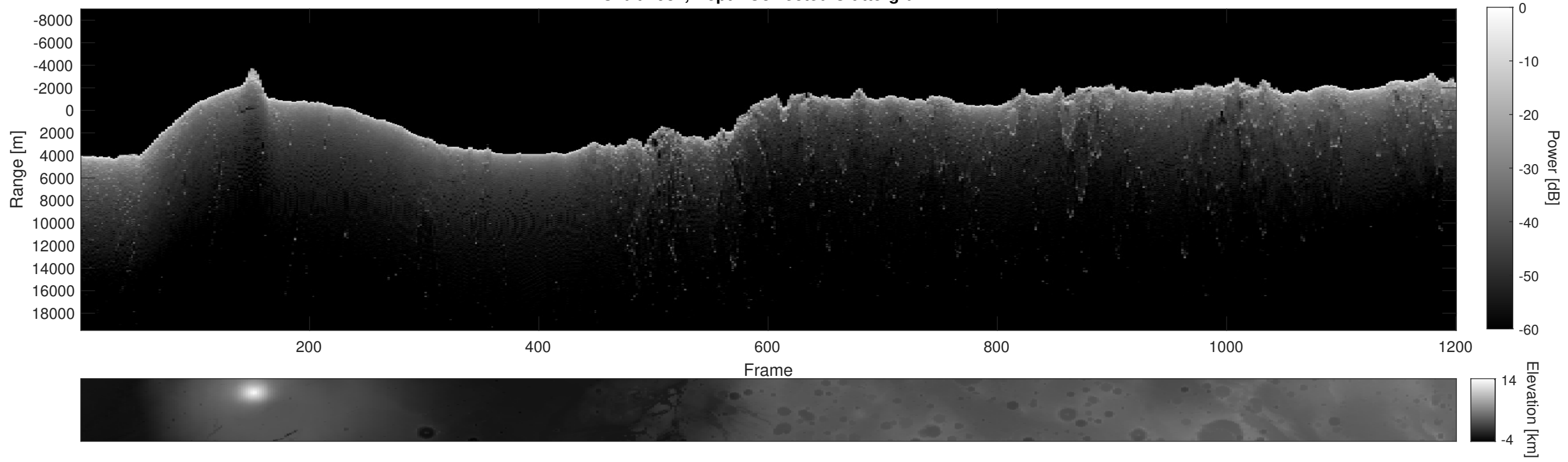
Orbit 2984, Depth-Corrected Cluttergram
