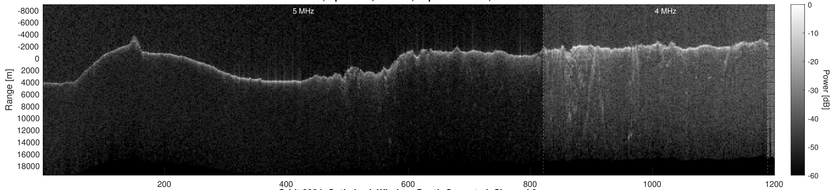
Orbit 2984, Optimized, Window, Depth-Corrected, Channel 2
