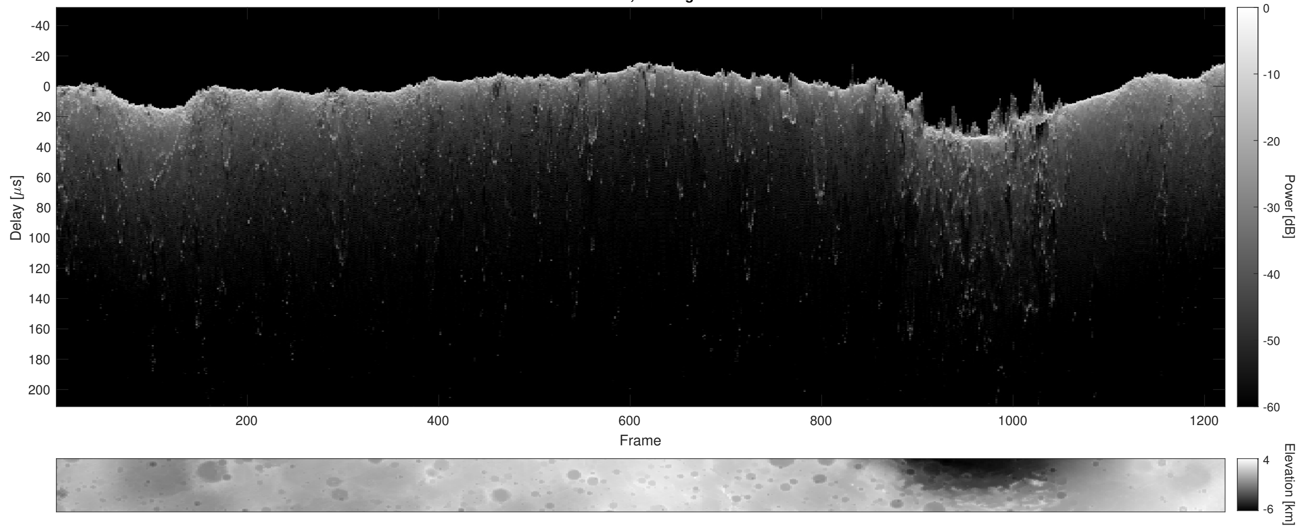
Orbit 2985, Cluttergram
