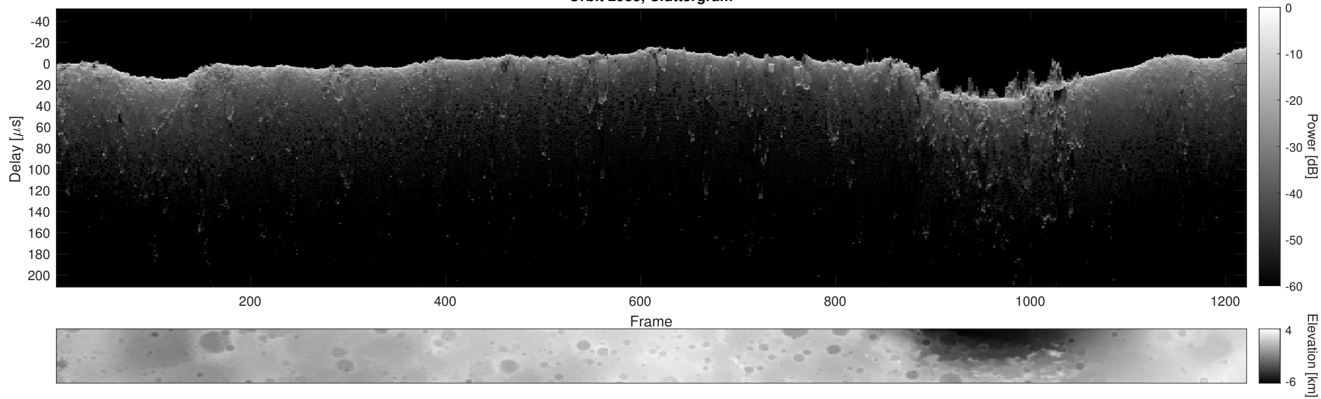
Orbit 2985, Cluttergram
