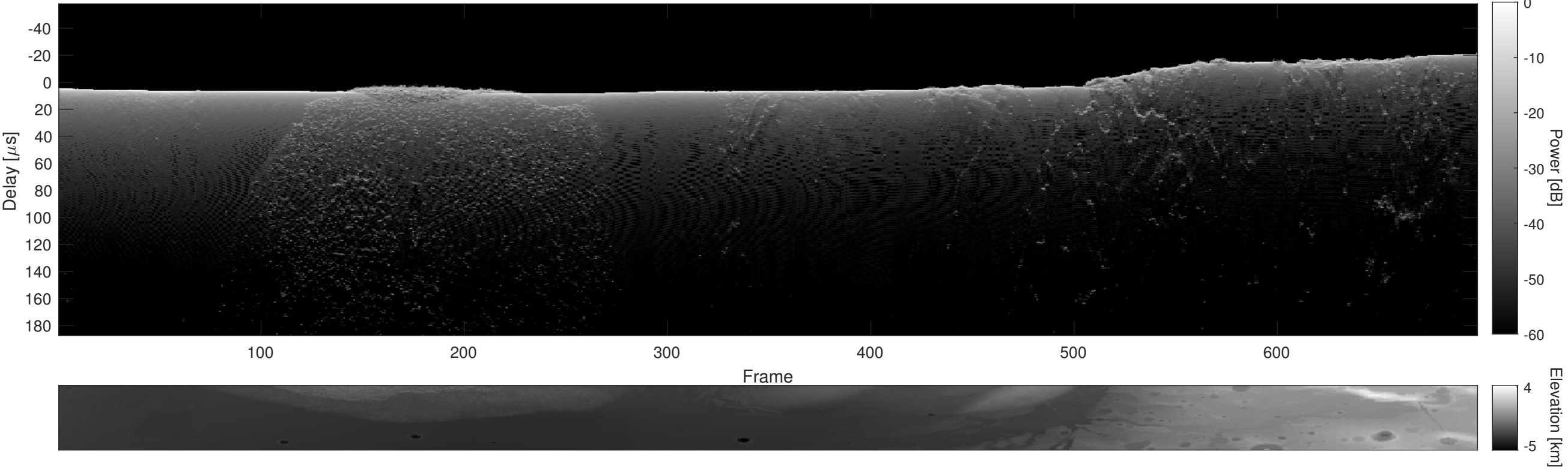
Orbit 2987, Cluttergram
