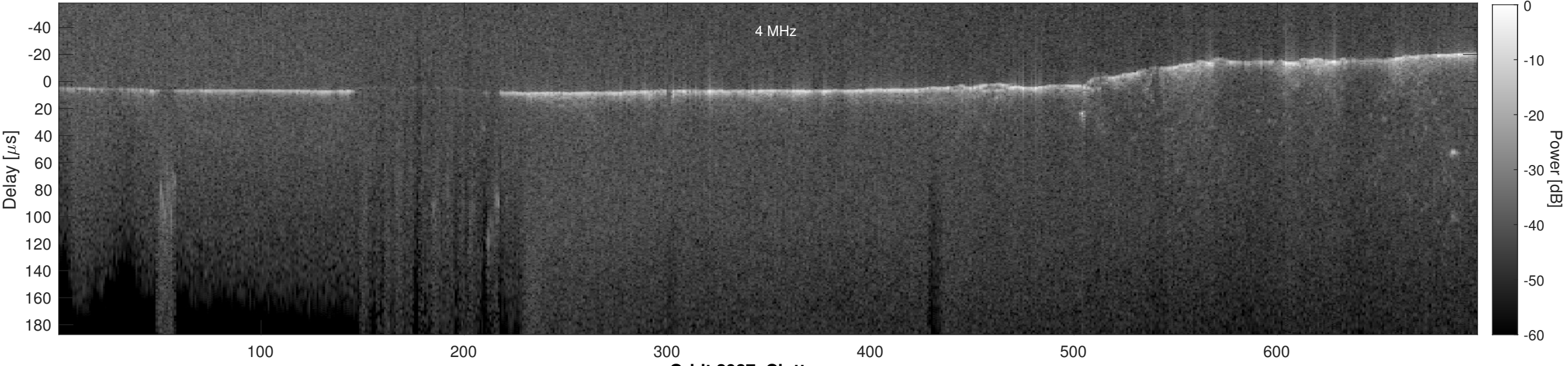
Orbit 2987, Cluttergram
