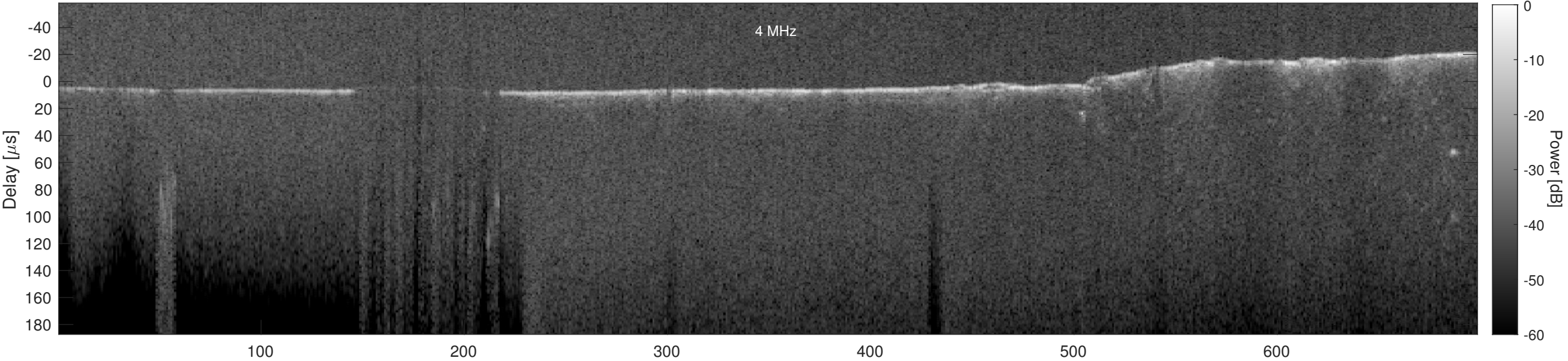
Orbit 2987, Cluttergram
