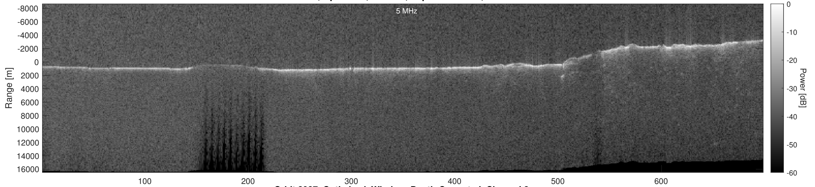
Orbit 2987, Optimized, Window, Depth-Corrected, Channel 2
