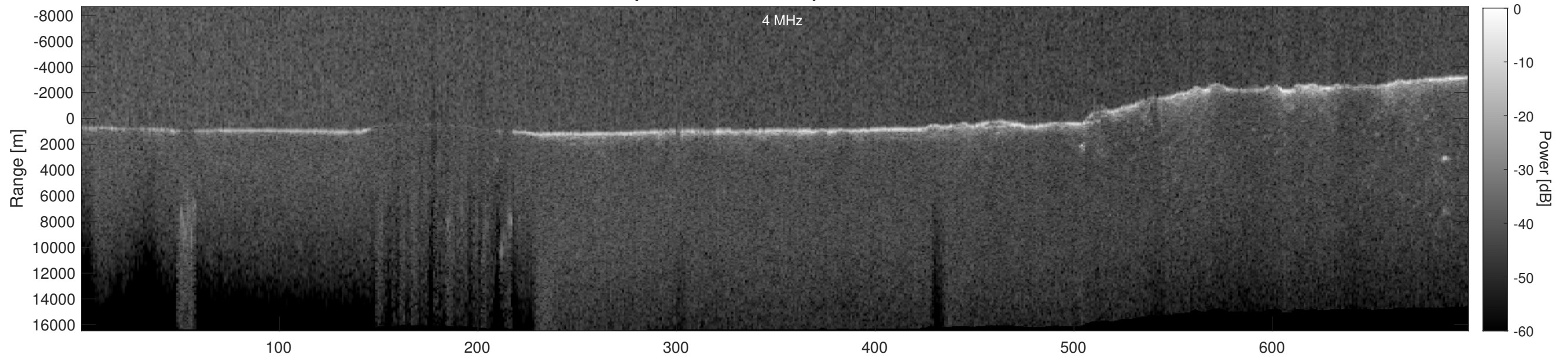
Orbit 2987, Depth-Corrected Cluttergram
