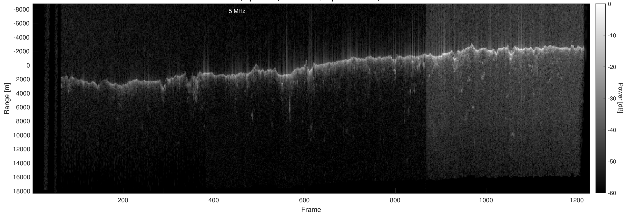
Orbit 2989, Optimized, No Window, Depth-Corrected, Channel 2
