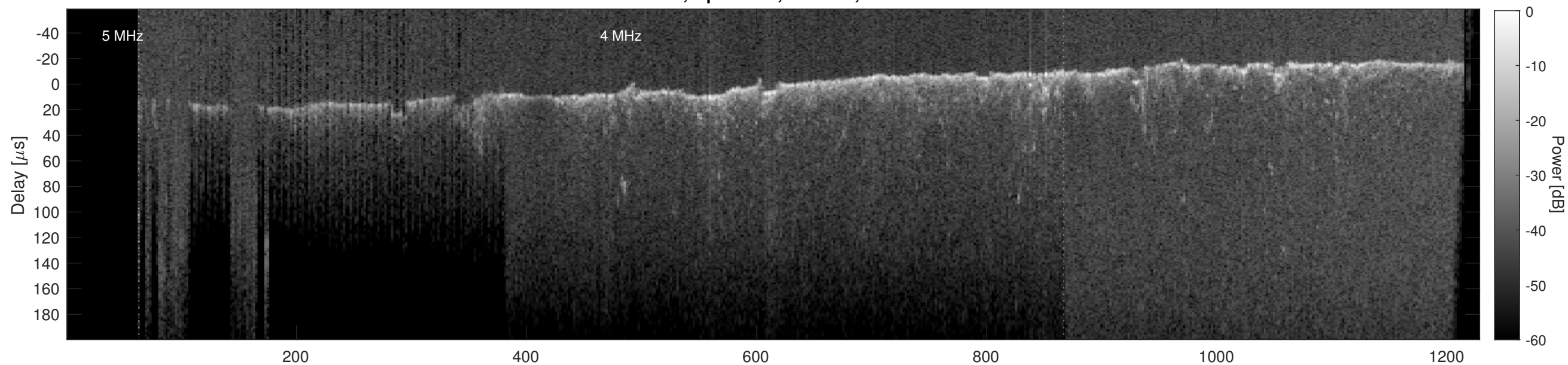
Orbit 2989, Cluttergram
