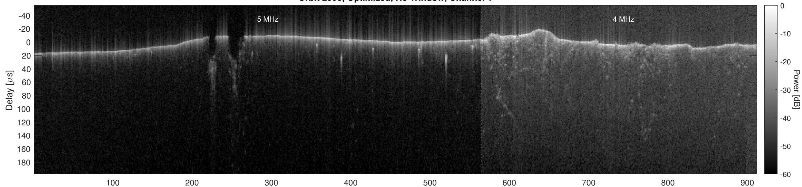
Orbit 2990, Optimized, No Window, Channel 2
