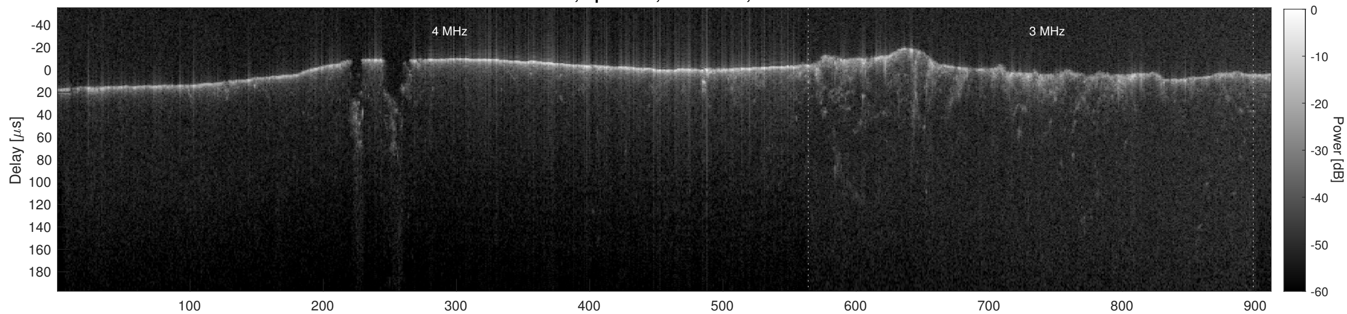
Orbit 2990, Cluttergram
