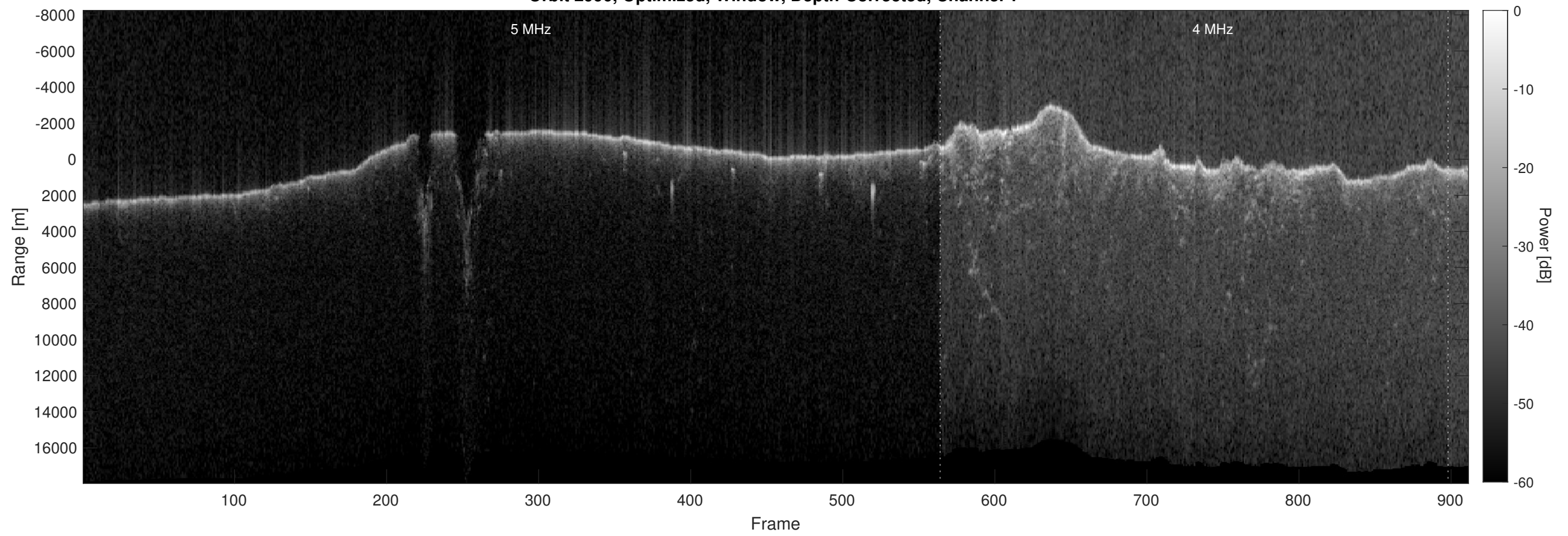
Orbit 2990, Optimized, Window, Depth-Corrected, Channel 2
