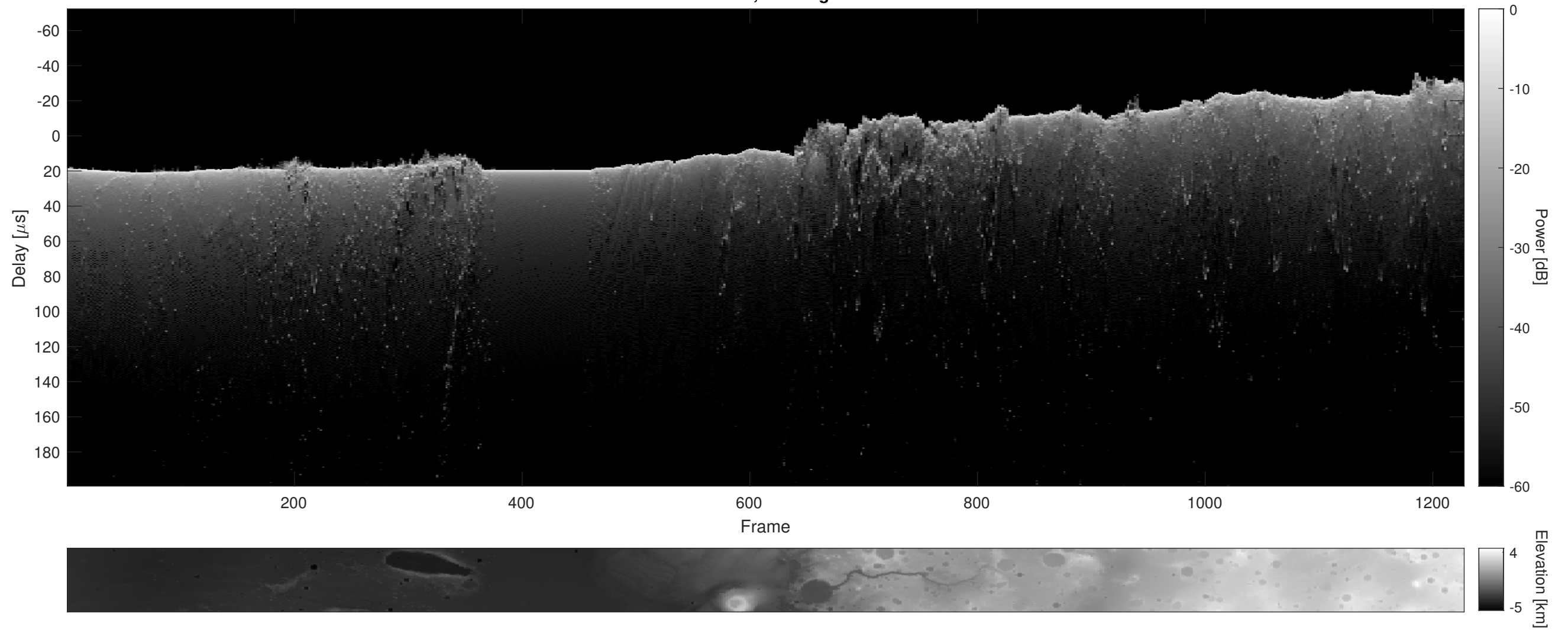
Orbit 2991, Cluttergram
