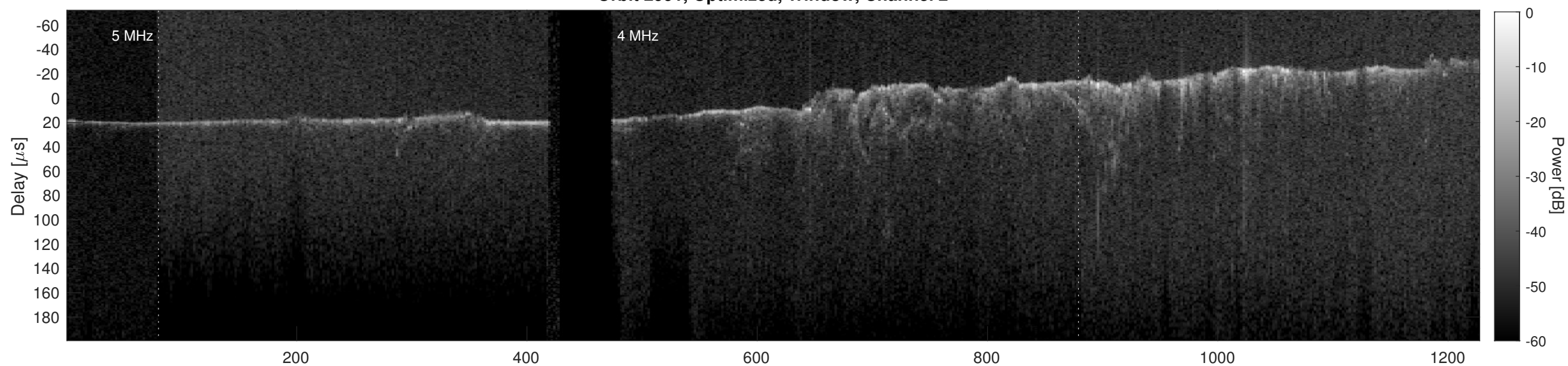
Orbit 2991, Cluttergram
