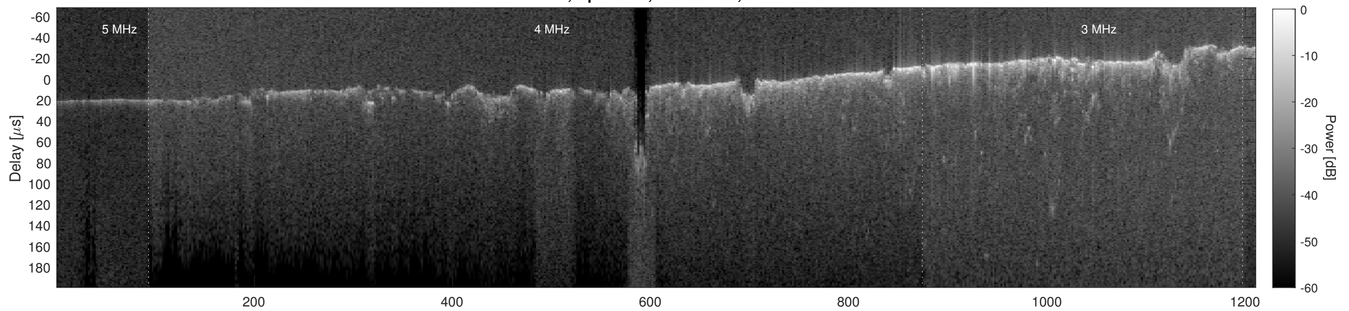
Orbit 2993, Cluttergram
