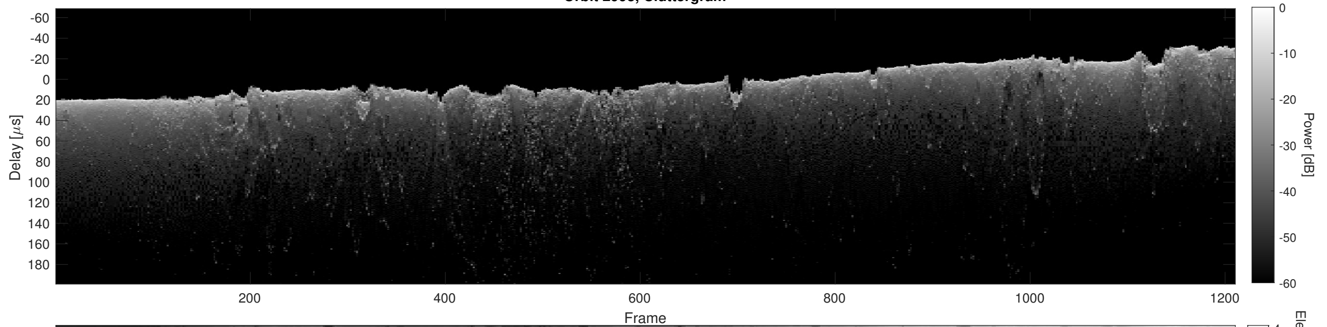
Orbit 2993, Cluttergram
