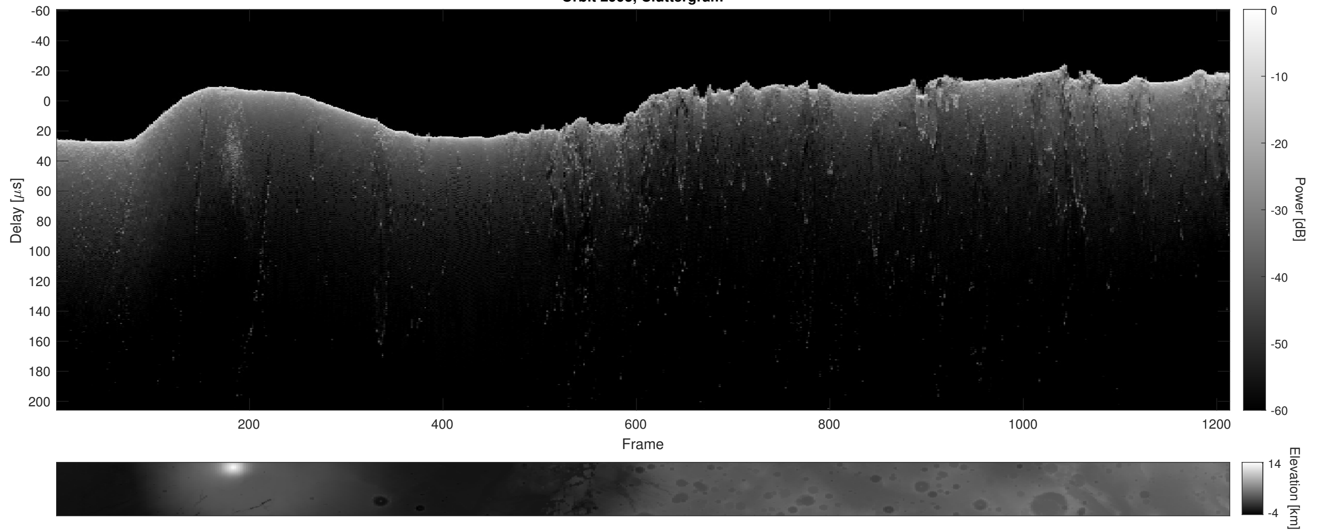
Orbit 2995, Cluttergram
