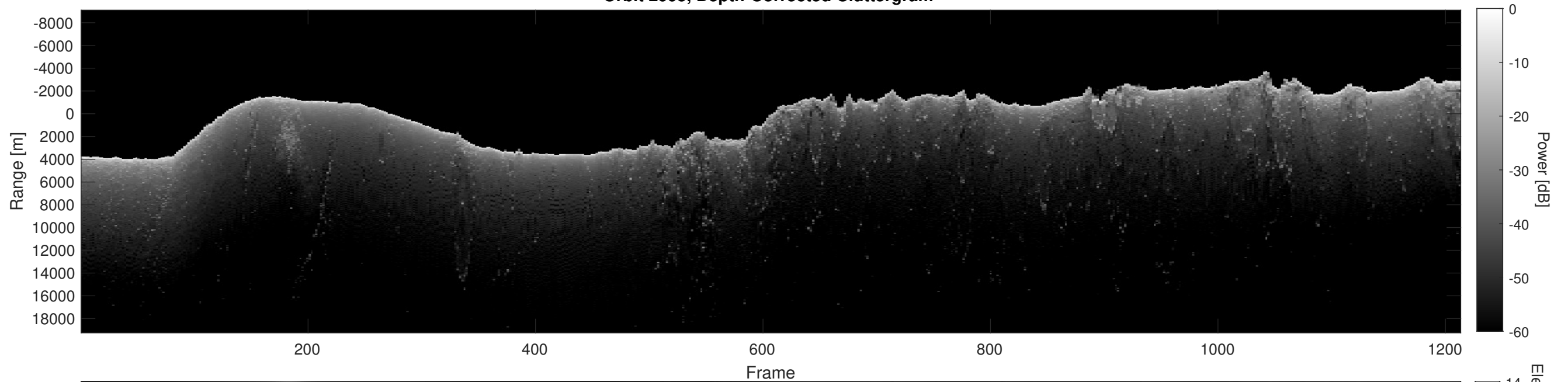
Orbit 2995, Depth-Corrected Cluttergram
