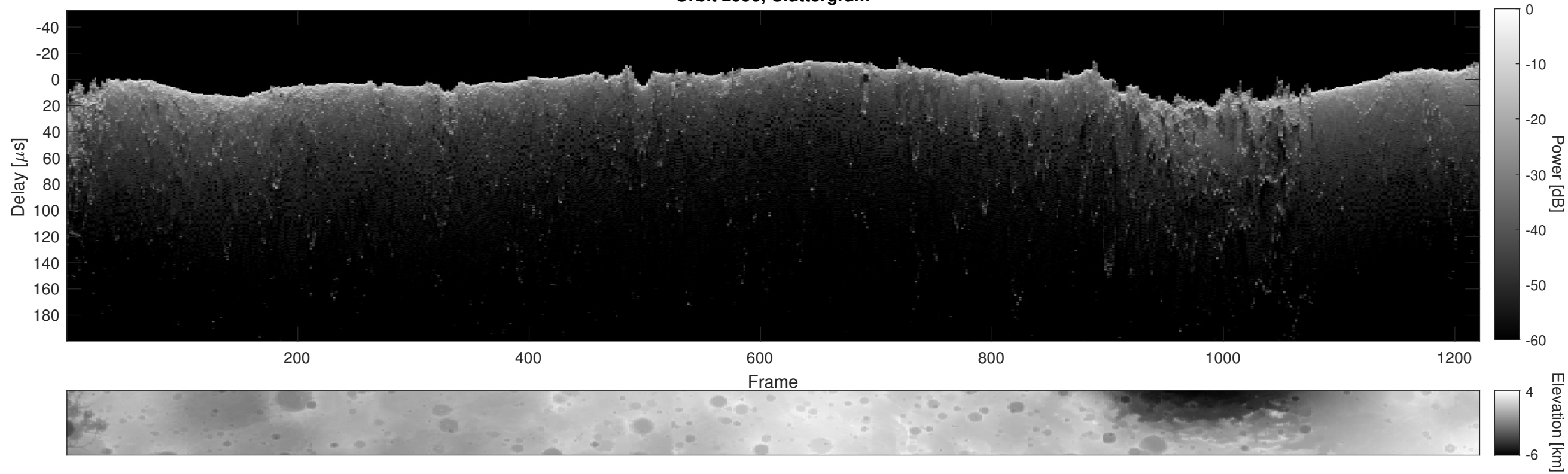
Orbit 2996, Cluttergram
