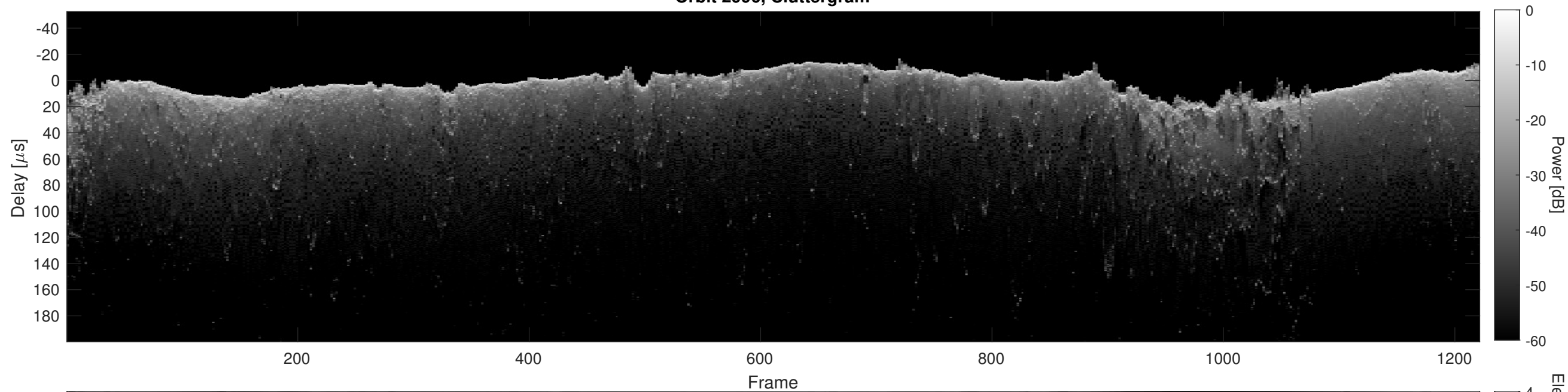
Orbit 2996, Cluttergram
