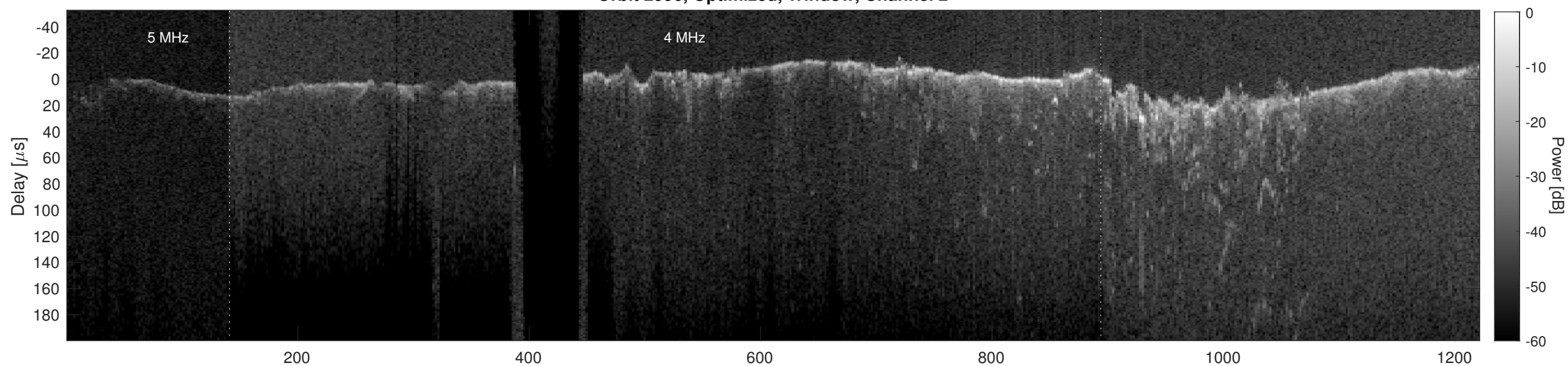
Orbit 2996, Cluttergram
