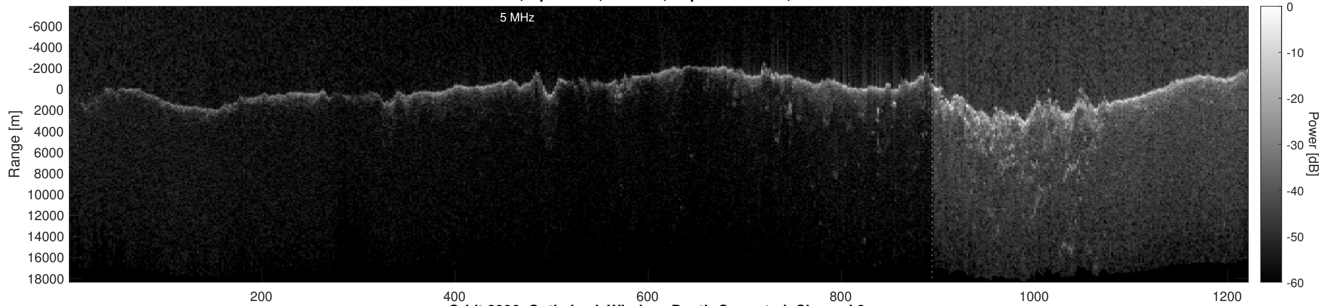
Orbit 2996, Optimized, Window, Depth-Corrected, Channel 2
