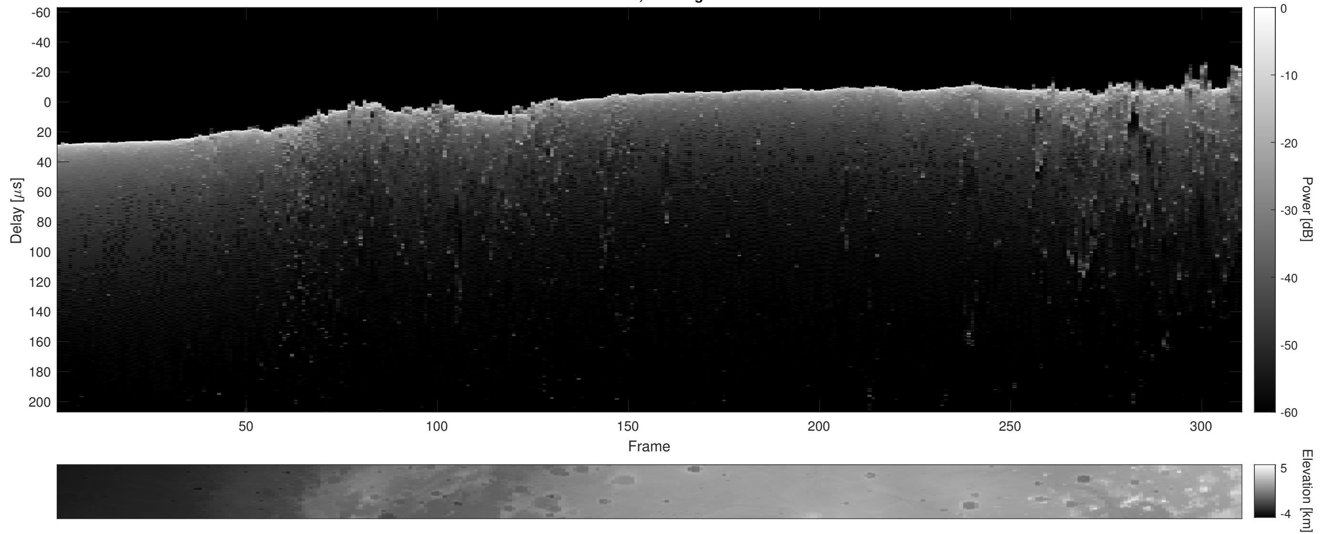
Orbit 2999, Cluttergram
