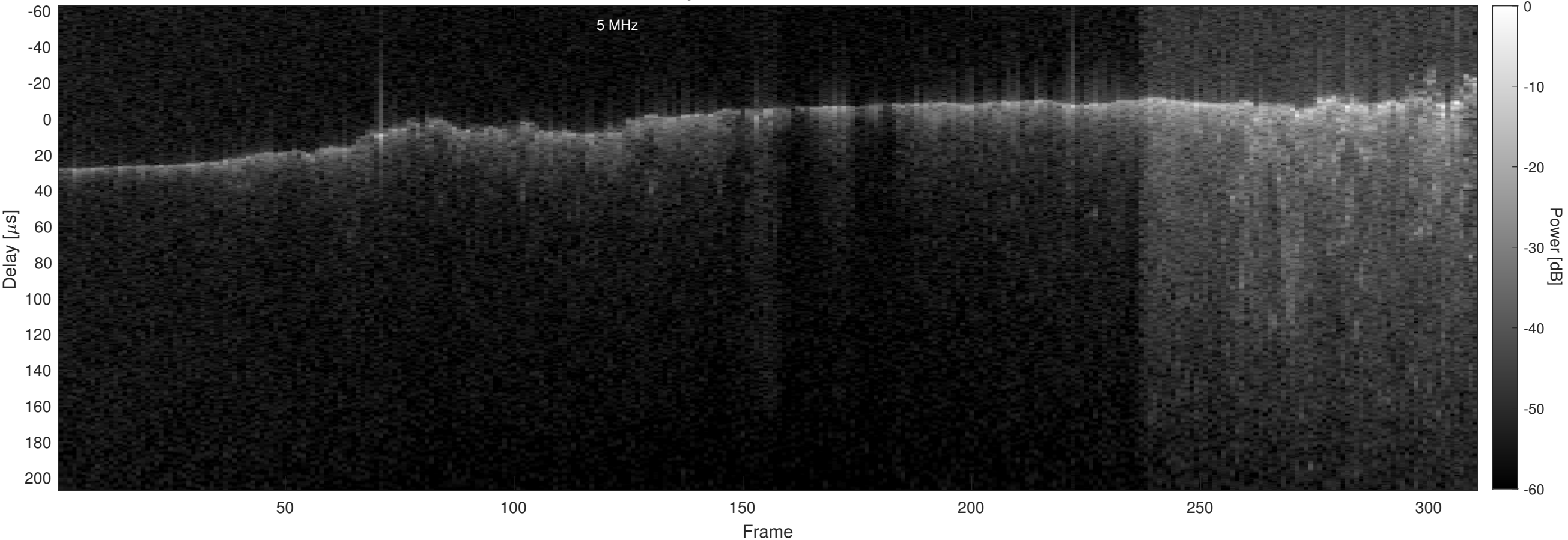
Orbit 2999, Optimized, No Window, Channel 2
