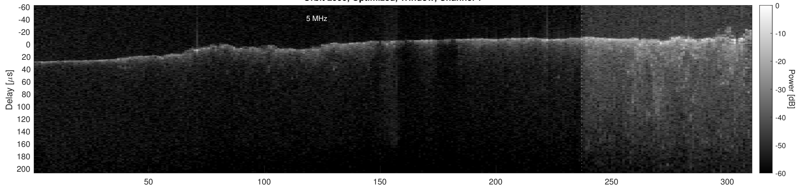
Orbit 2999, Optimized, Window, Channel 2
