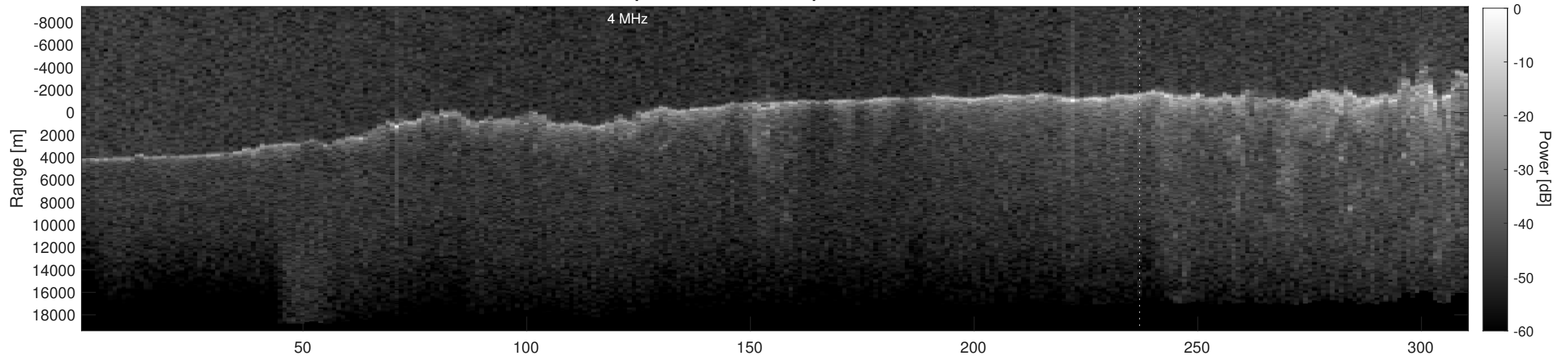
Orbit 2999, Depth-Corrected Cluttergram
