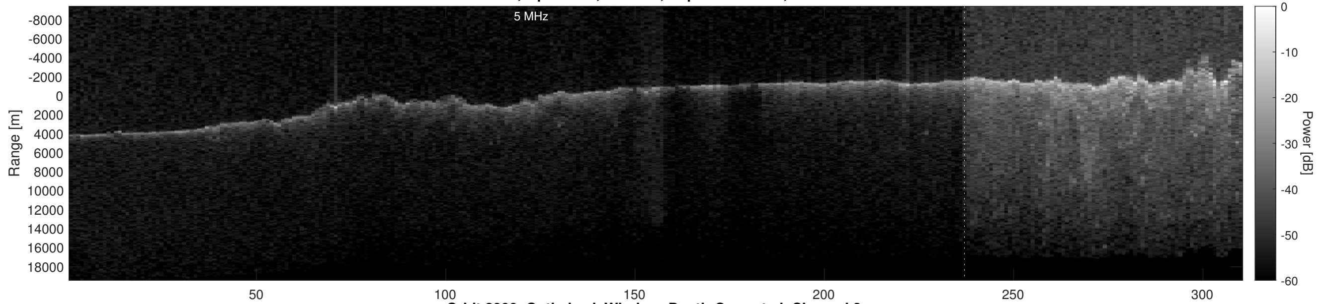
Orbit 2999, Optimized, Window, Depth-Corrected, Channel 2
