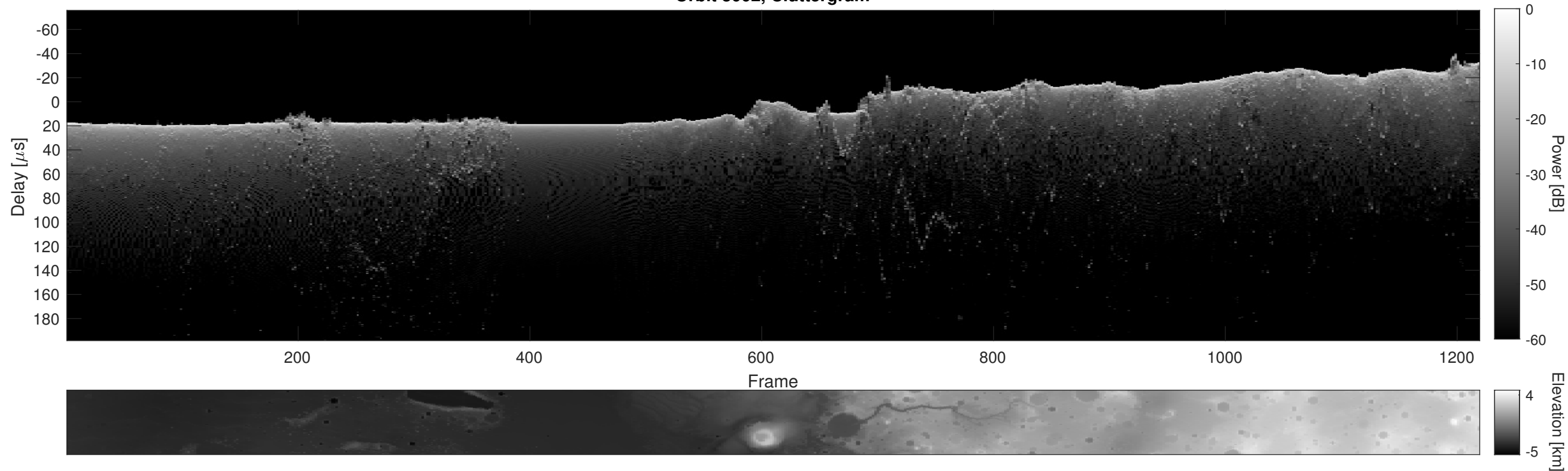
Orbit 3002, Cluttergram
