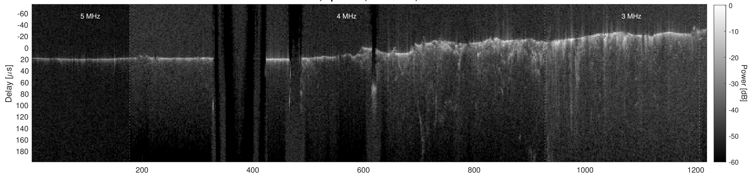
Orbit 3002, Cluttergram
