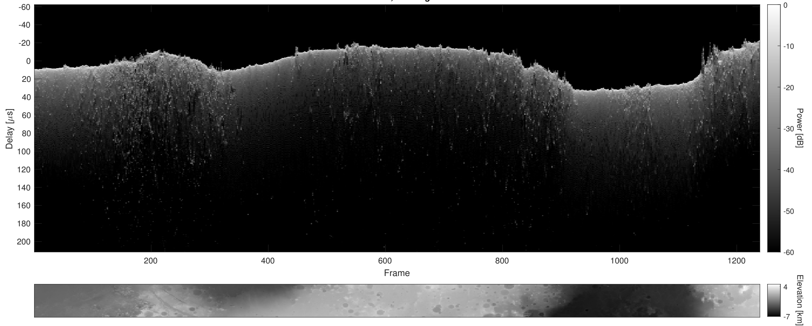
Orbit 3003, Cluttergram
