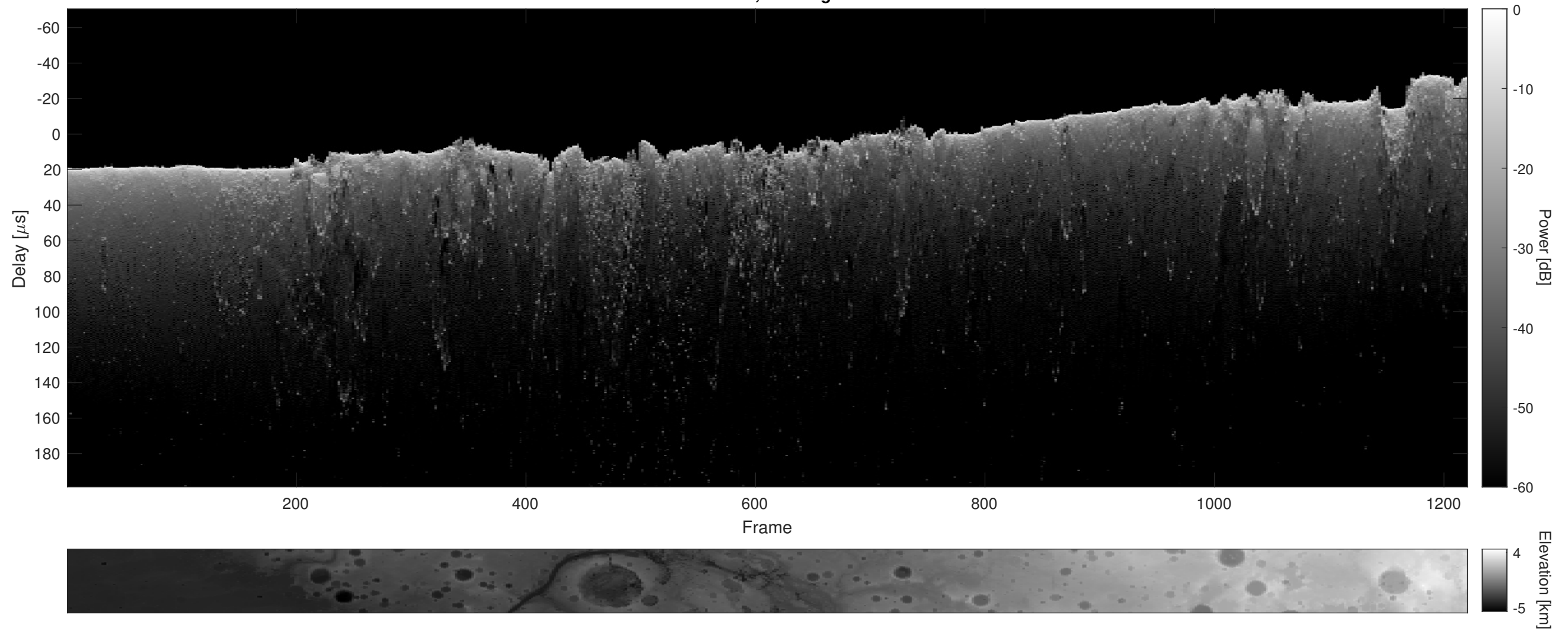
Orbit 3004, Cluttergram
