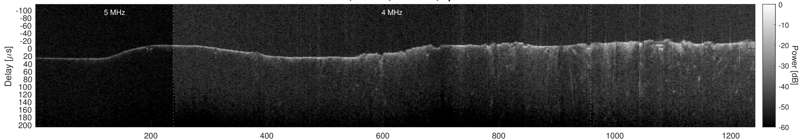
Orbit 3006, Cluttergram
