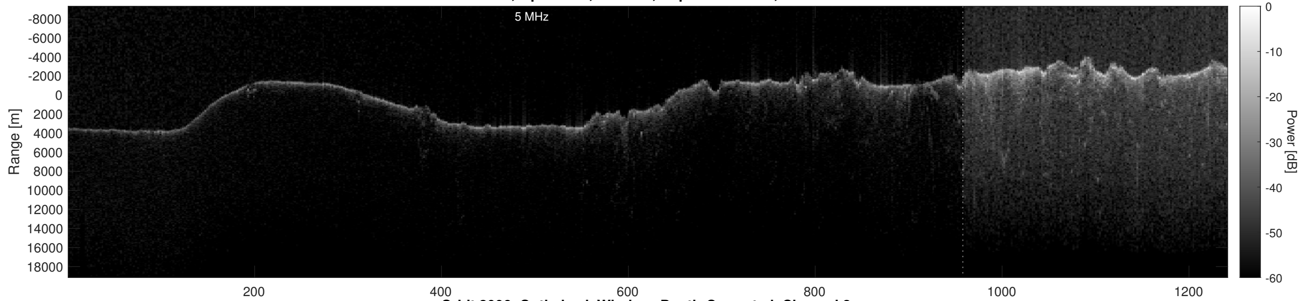
Orbit 3006, Optimized, Window, Depth-Corrected, Channel 2
