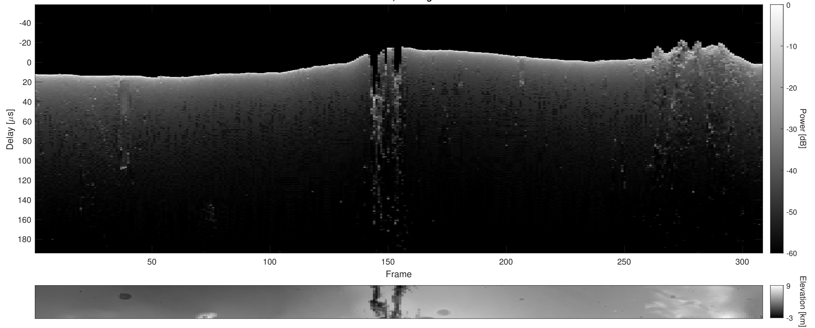
Orbit 3023, Cluttergram
