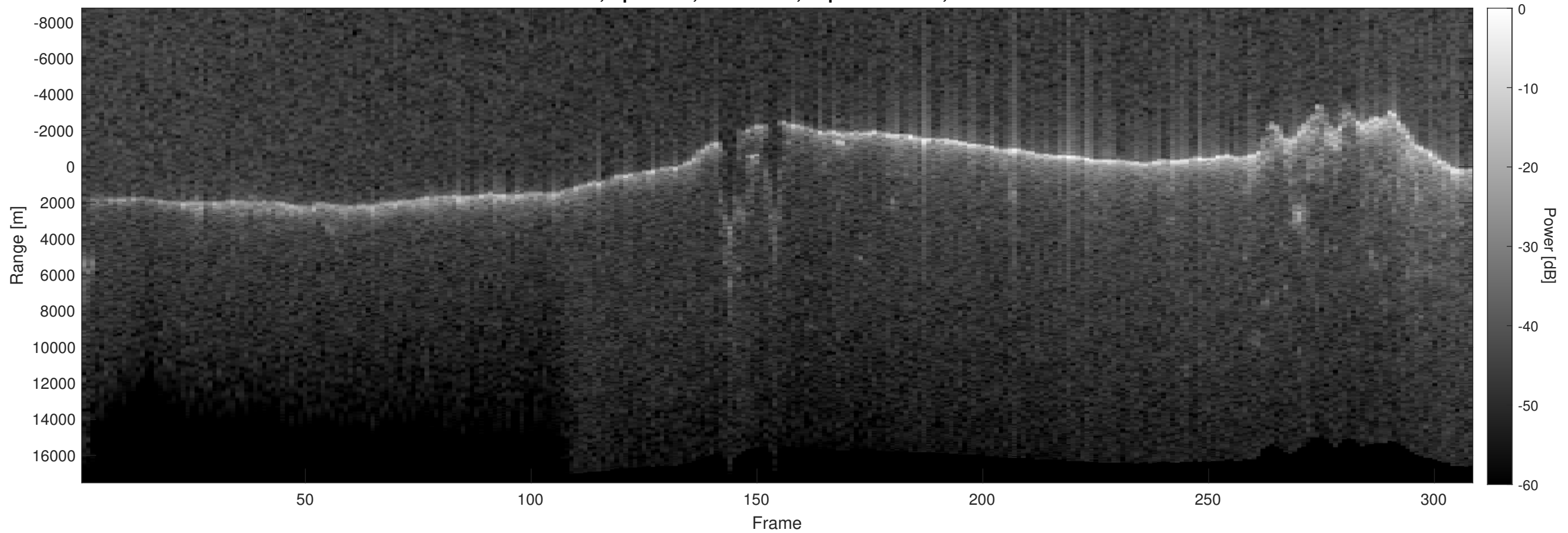
Orbit 3023, Optimized, No Window, Depth-Corrected, Channel 2
