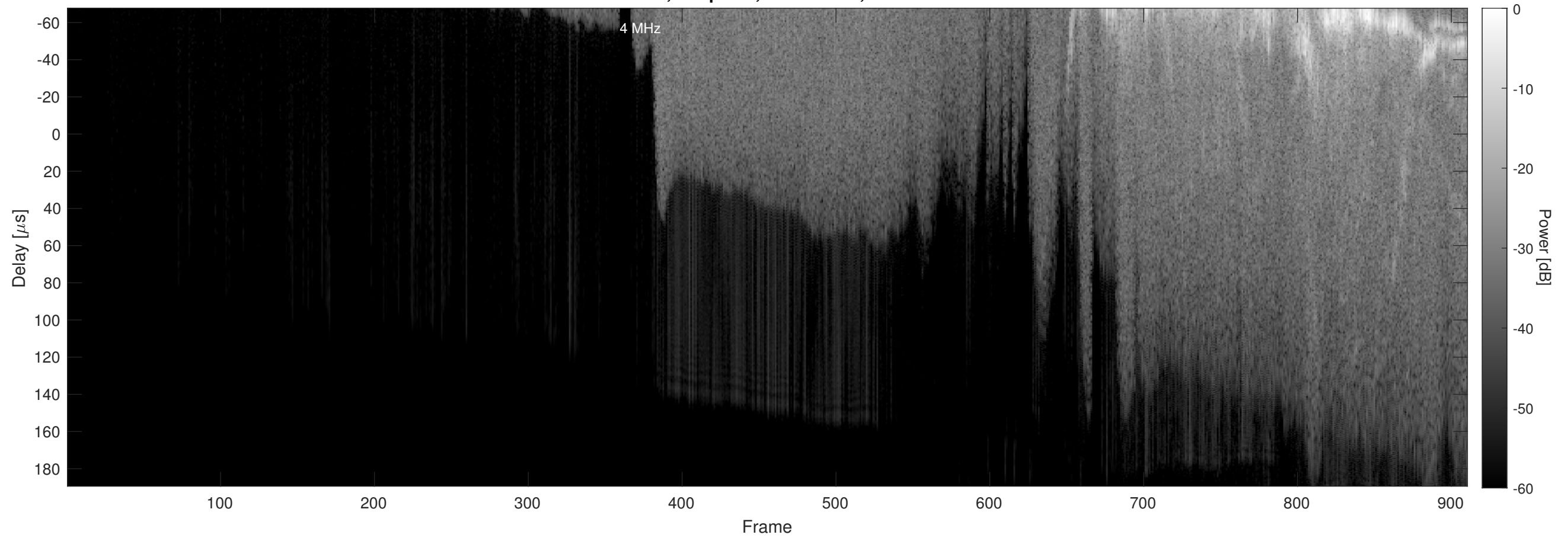
Orbit 3024, Chapman, No Window, Channel 2
