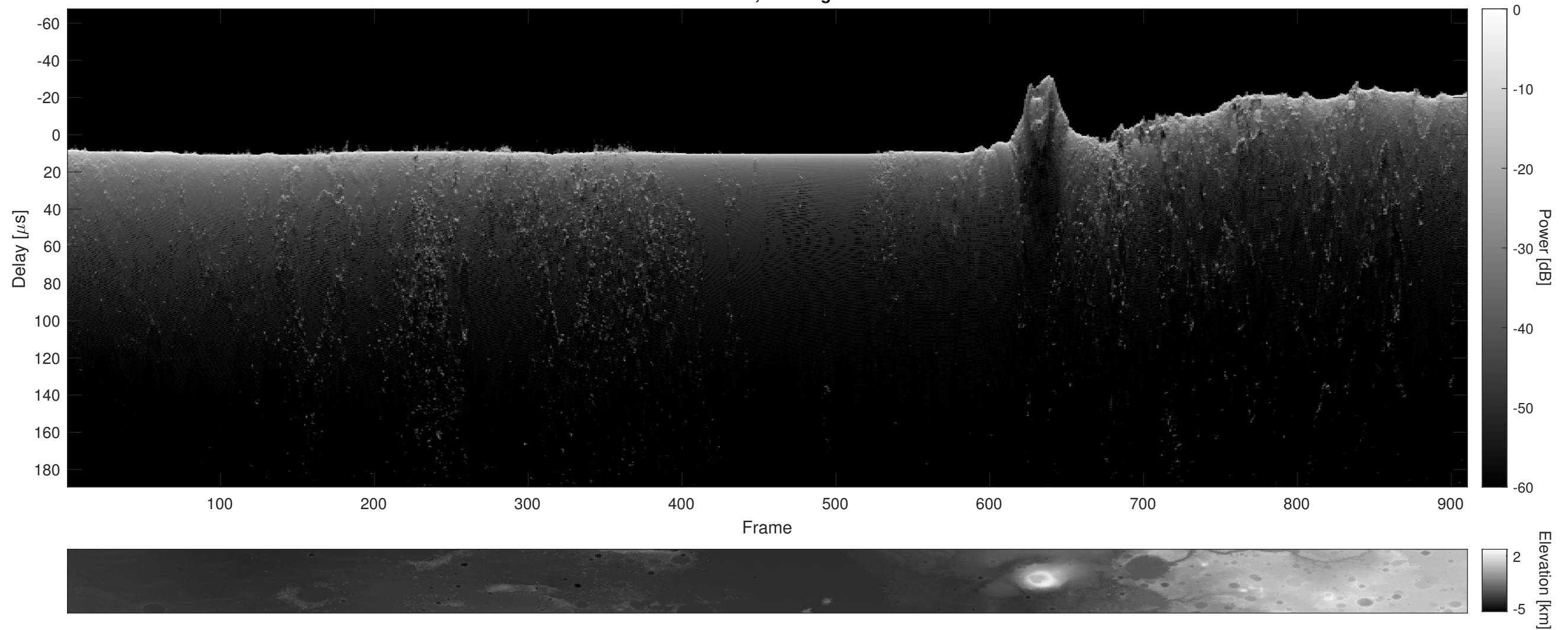
Orbit 3024, Cluttergram
