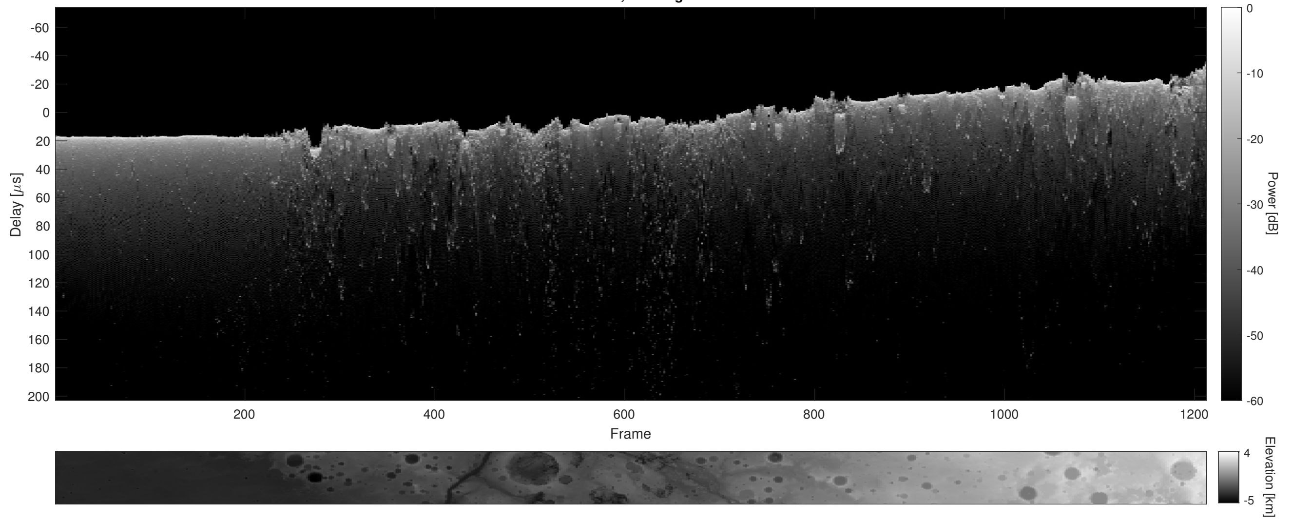
Orbit 3026, Cluttergram
