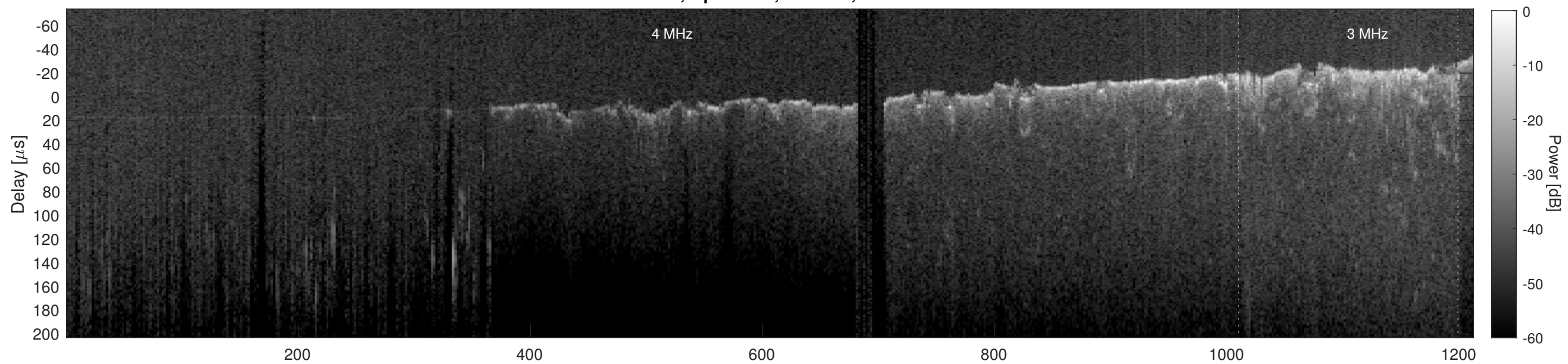
Orbit 3026, Cluttergram
