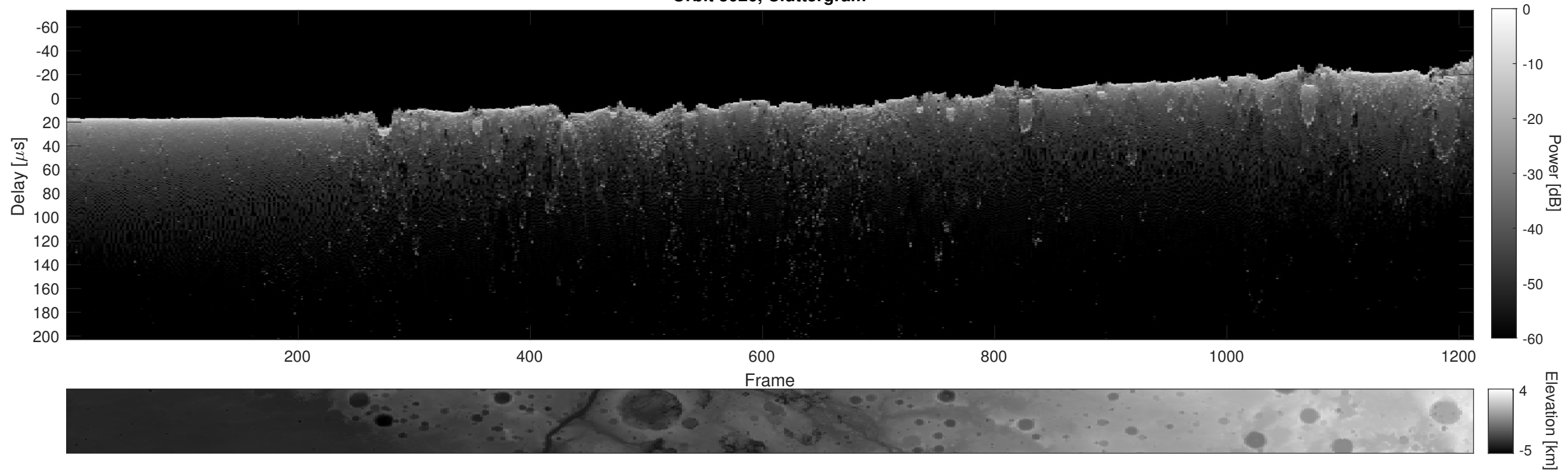
Orbit 3026, Cluttergram
