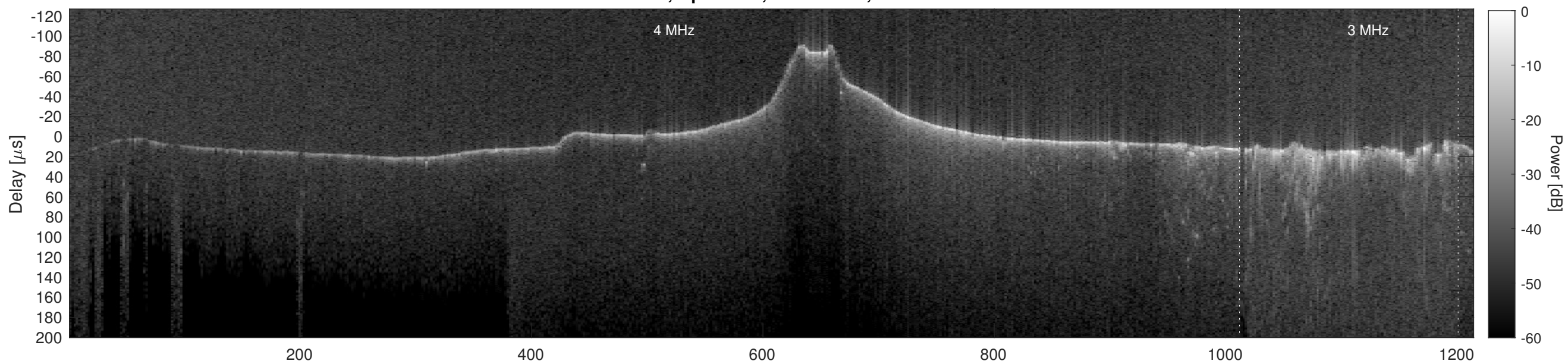
Orbit 3027, Cluttergram
