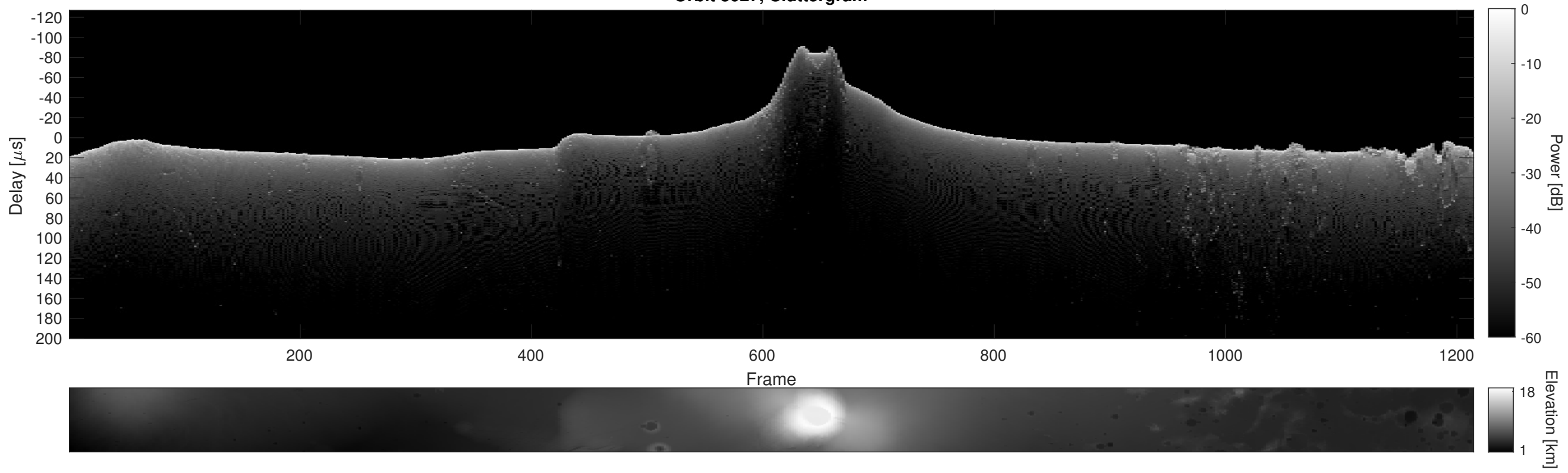
Orbit 3027, Cluttergram
