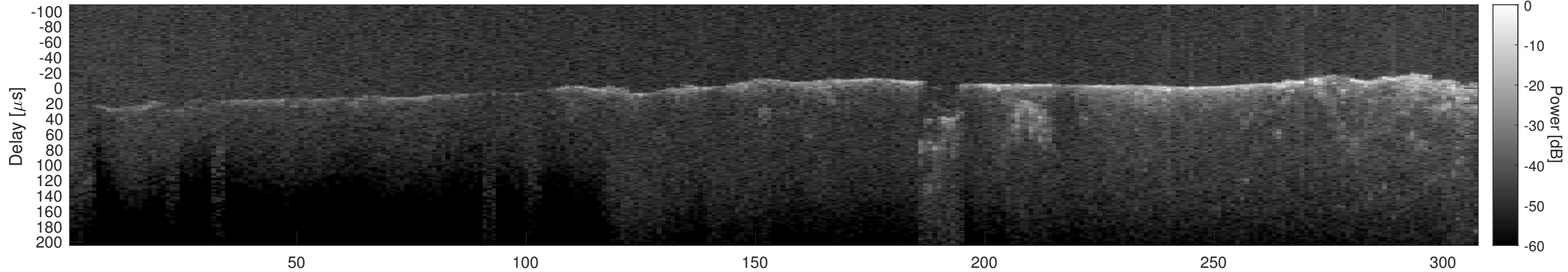
Orbit 3030, Cluttergram
